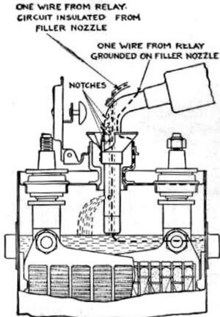
Diagram showing circuit of Electric Filler. Note that when solution reaches the correct level the end of filler nozzle just touches the solution, thereby completing the circuit and causing the bell to ring. The notches on the handle of filler give correct adjustment for different types of cells.
